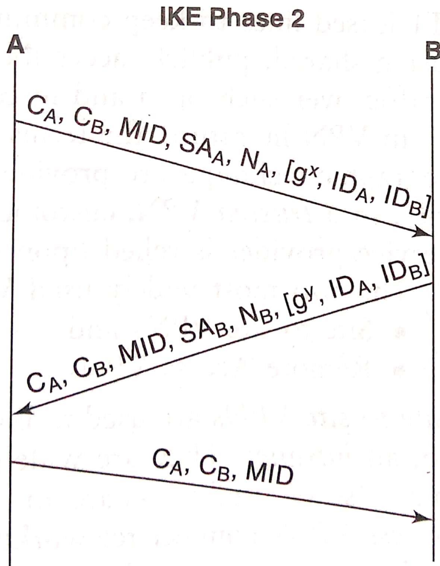
Figure 13.6 IKE phase 2
