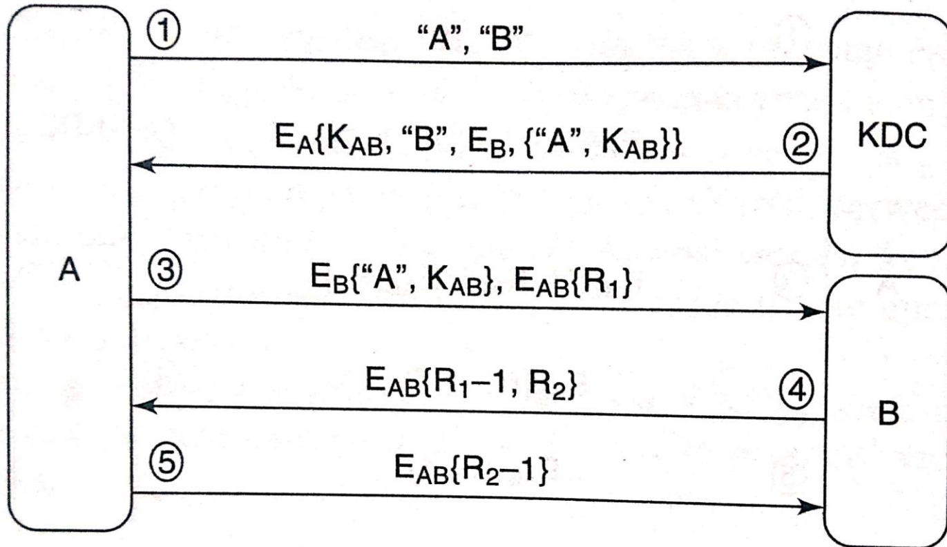
(a) Preliminary version 2
