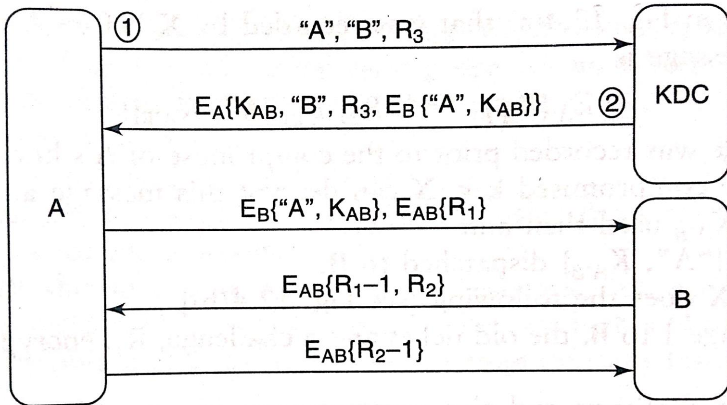
(a) : Preliminary version 3
