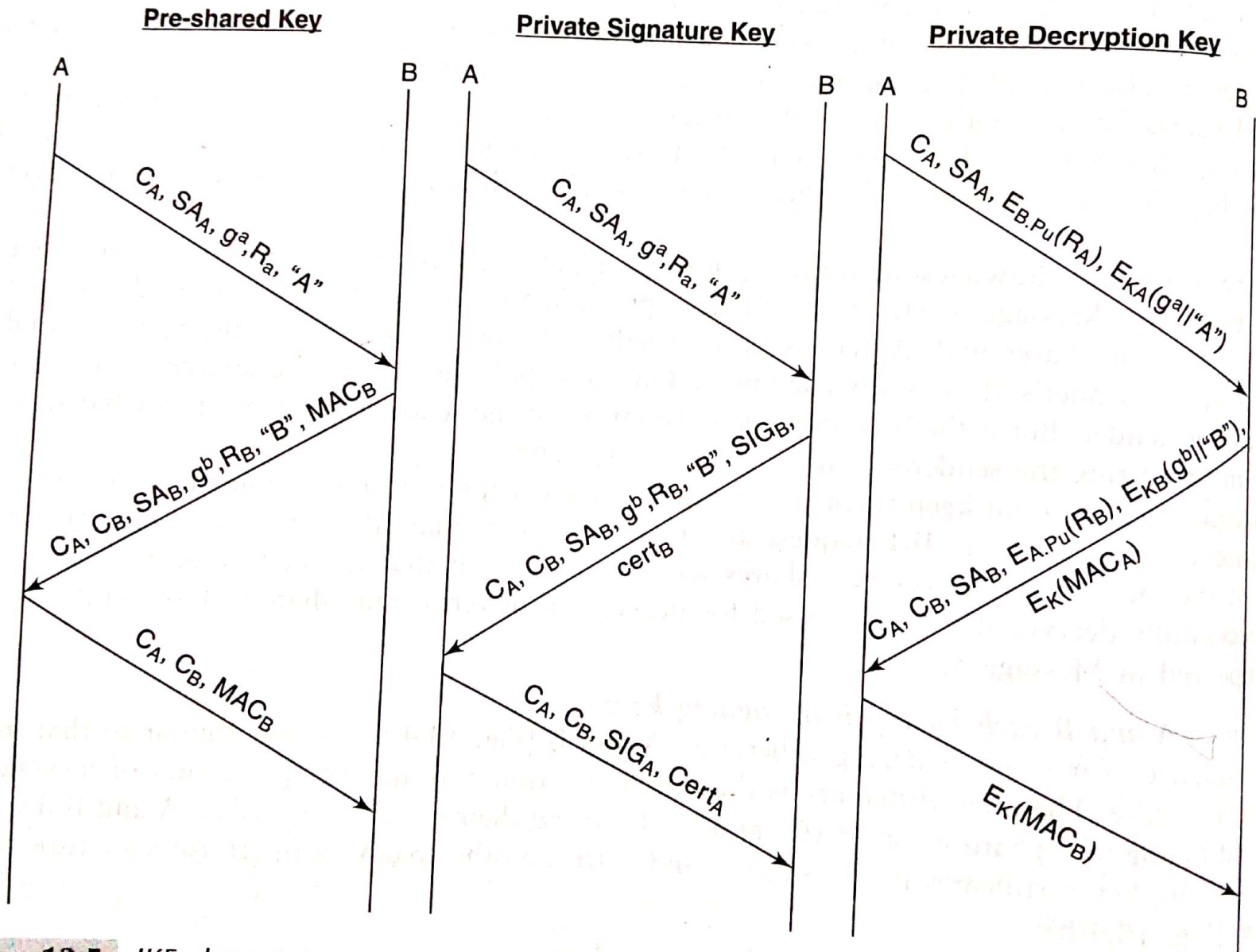
Figure 13.5 IKE phase 1 (aggressive mode)
