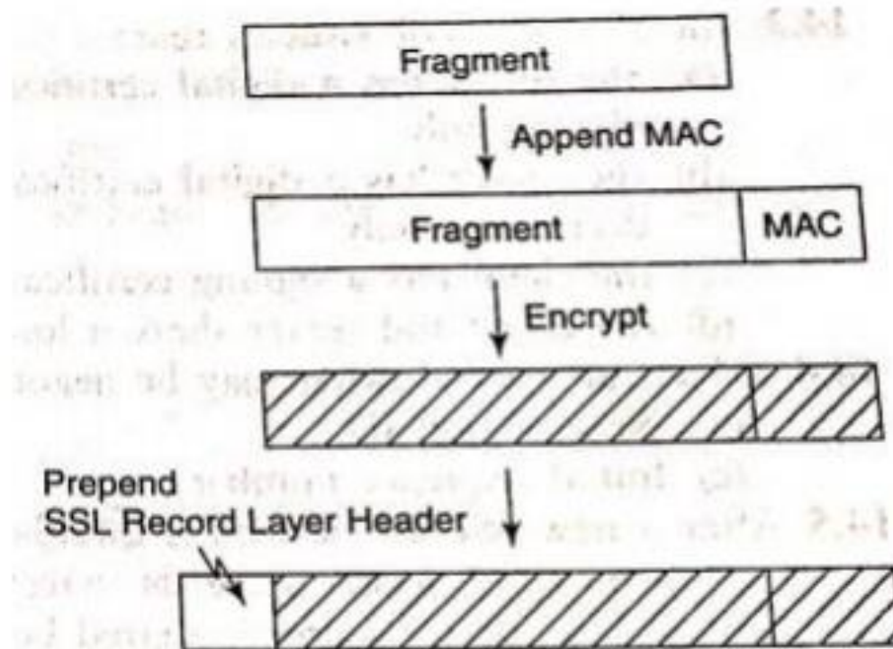
Figure 14.3 Function of the SSL record layer protocol
