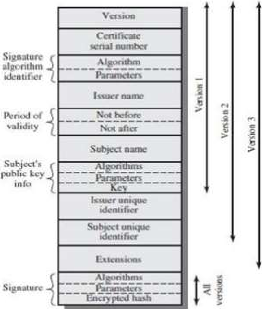
(a) X.509 certificate
