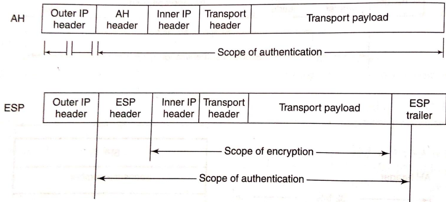
Figure 13.2 AH and ESP in tunnel mode
