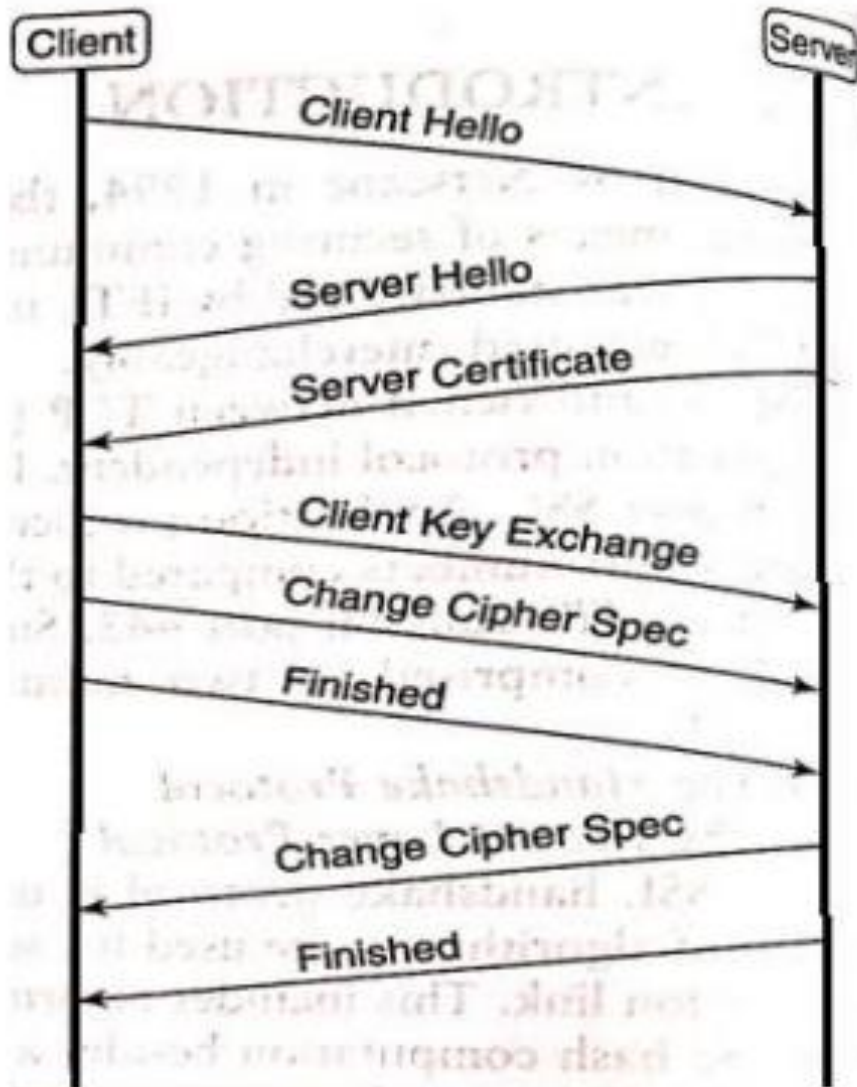
Figure 14.2 SSL handshake
