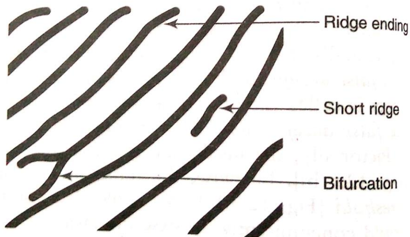
Figure 12.10 Minutiae patterns
