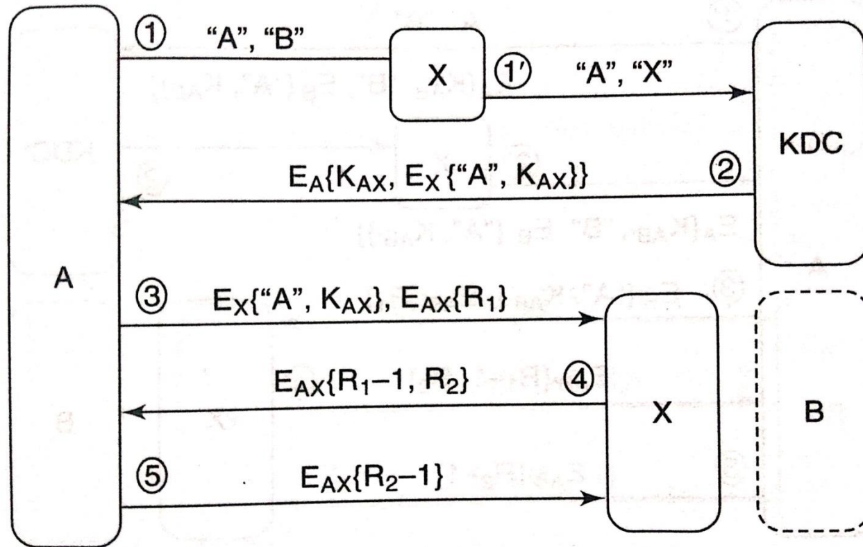
(b) : Man-in-the middle attack on preliminary version 1
