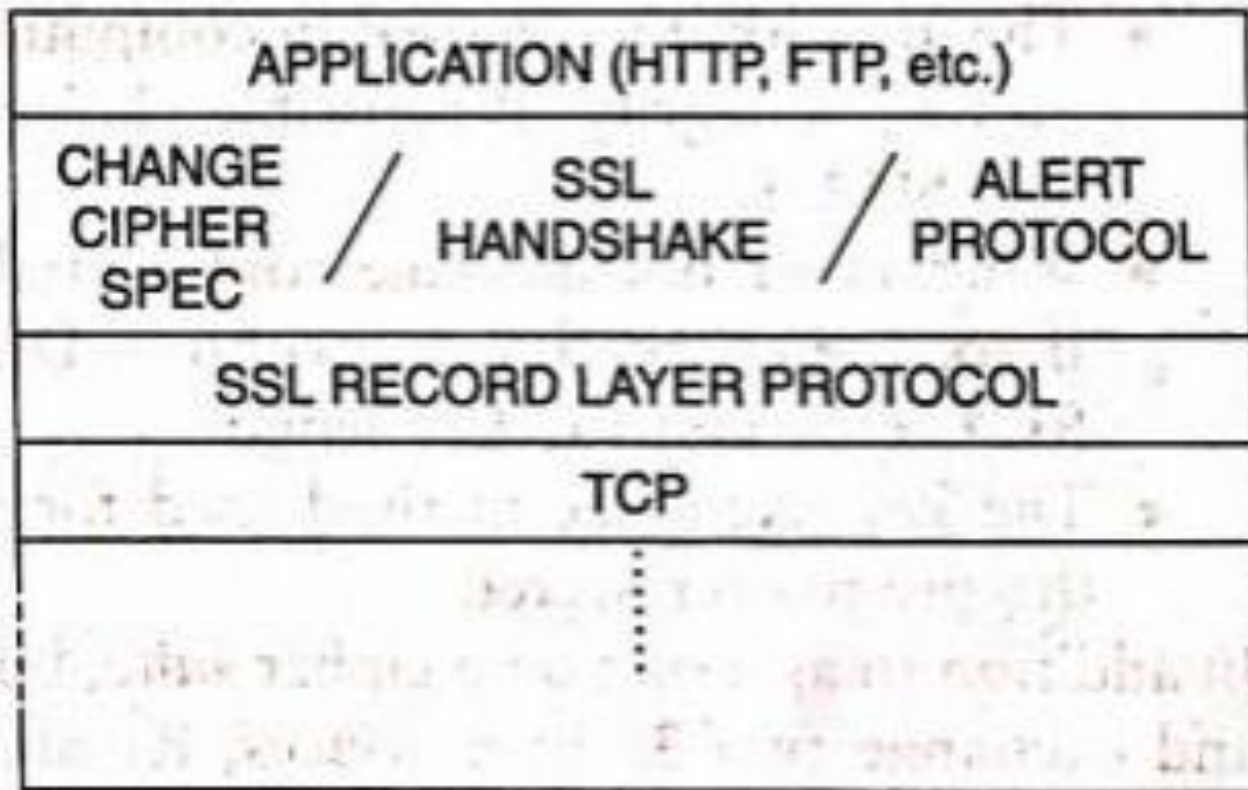
Figure 14.1 SSL on the protocol stack
