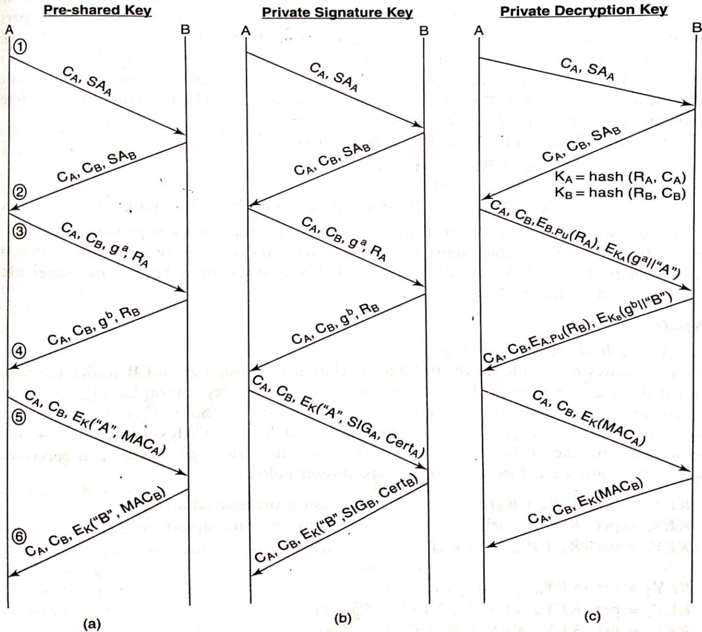
Figure 13.4 IKE phase 1 (main mode)
